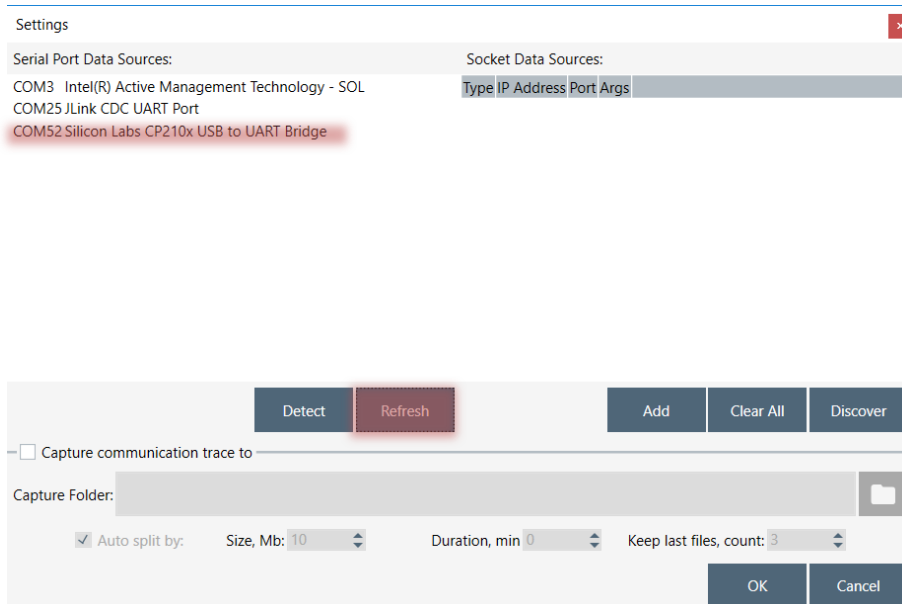
Figure 7: Settings Windows
