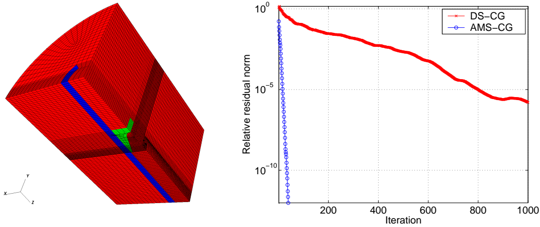
Fig. 6.4. Initial mesh and (logarithmic) converge history plot for a MHD simulation.
