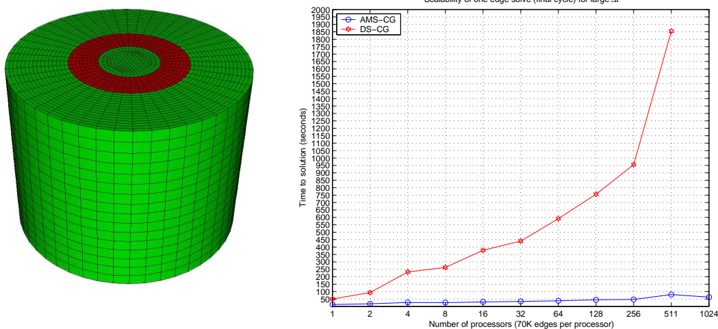
Fig. 6.3. Initial mesh and time to solution for the copper wire model.
