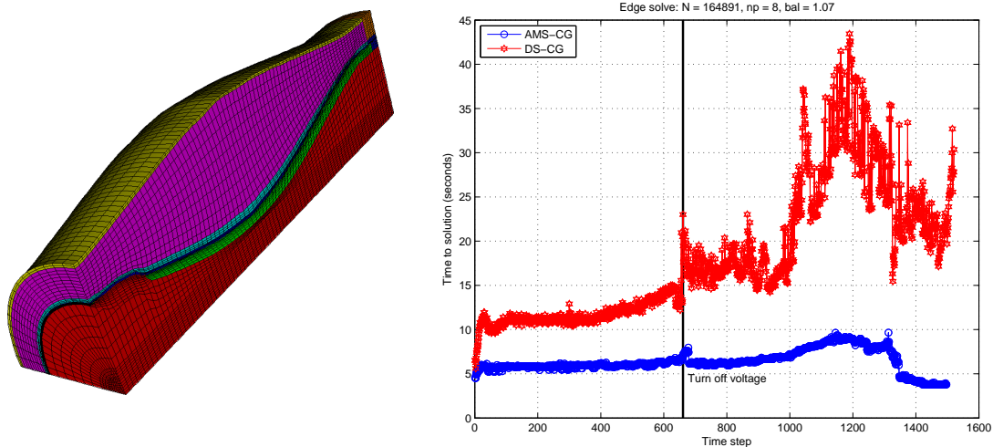
Fig. 6.5. The magnetic flux compression generator mesh in the middle of the calculation (left) and the time needed for the Maxwell solves at each time step during the simulation (right).
