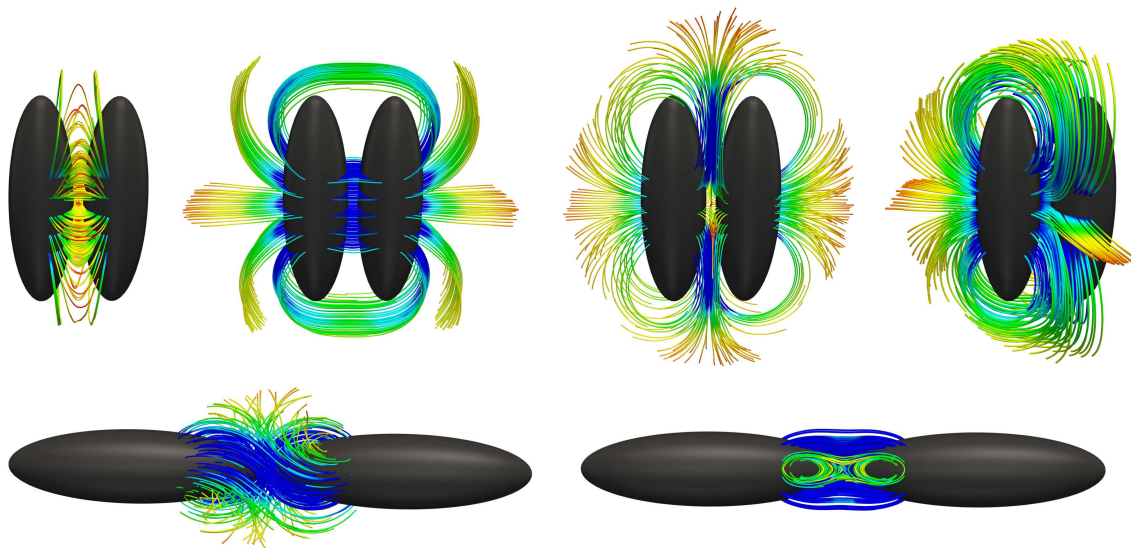
Fig. 6.6. Streamlines of the magnetic fields generated by interactions between two magnetic orbs.
